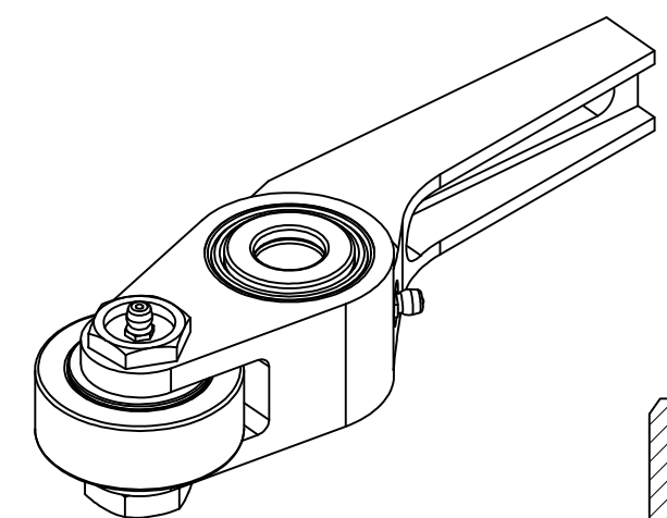
ISOMETRIC ASSMBLED VIEW (FOR REFERENCE ONLY)
