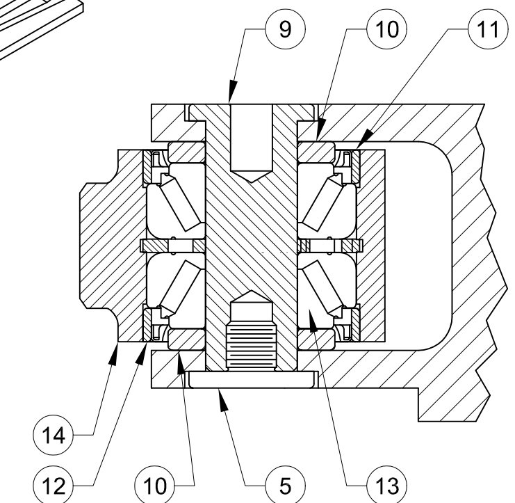
SECTION THRU BEARING ASSEMBLY
