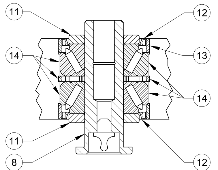
SECTION THRU BEARING ASSEMBLY
